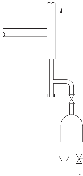
Figure LD-479-2. Drain trap draining air line drip pocket. Be sure to use a gate valve and blow down the assembly before installing trap.
