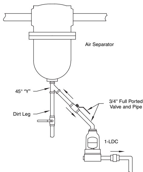
Figure LD-460-1. Typical Drain Trap Location
