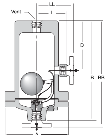
Figure LD-471-4. Model 71-315 forged steel snap action drain trap.
