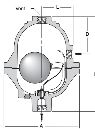
Figure LD-471-3. Model 71-A cast iron snap action drain trap.
