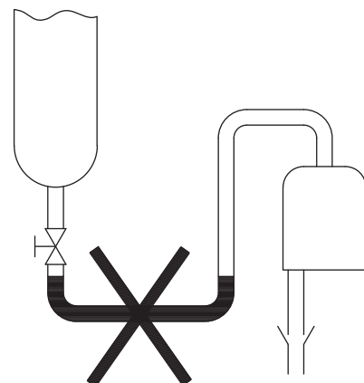
Figure LD-479-5. Do not install a ball float trap above the drip point or put a loop or pocket in the line to the trap. The water seal prevents air from leaving trap body and allowing liquid to enter.
