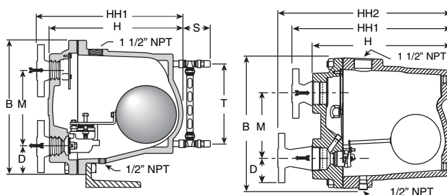
Figure LD-476-1. L and LS Series
