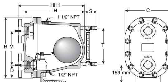
Figure LD-476-3. M and MS Series
