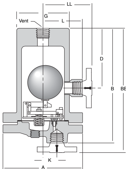
Figure LD-473-1. High leverage ball float drain trap.
