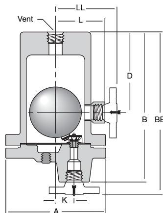
Figure LD-471-2. Model 21-312 forged steel fixed lever drain trap.
