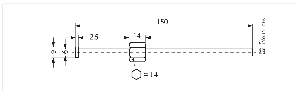
Weld nipple for KP-A
