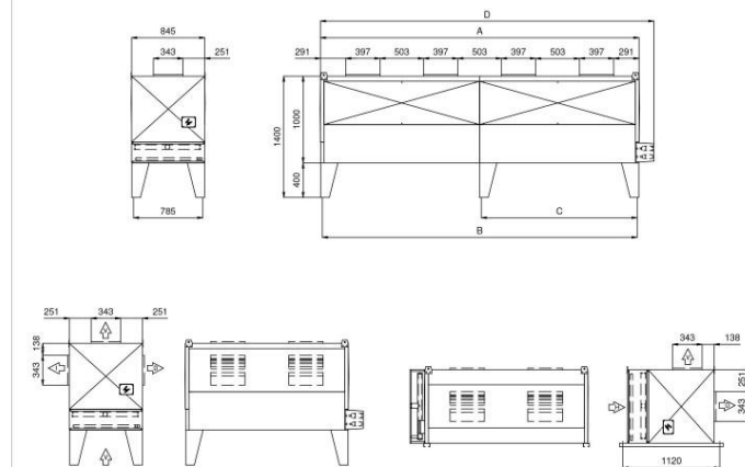
ESQUEMA GMC / GMC DRAWING
