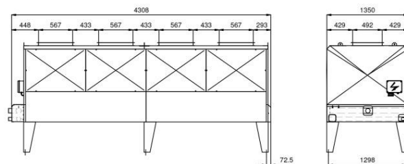
ESQUEMA GSC (TIPO 2) / GSC DRAWING (TYPE 2)
